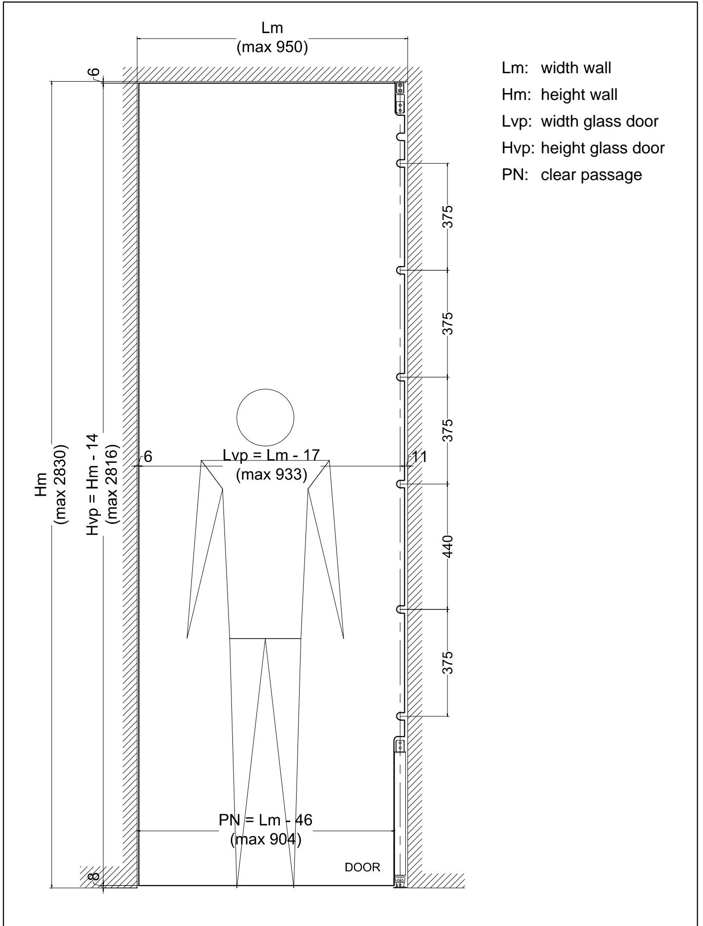
CT.D1.02 L ZENITH D1 - MAXIMUM DIMENSIONS
