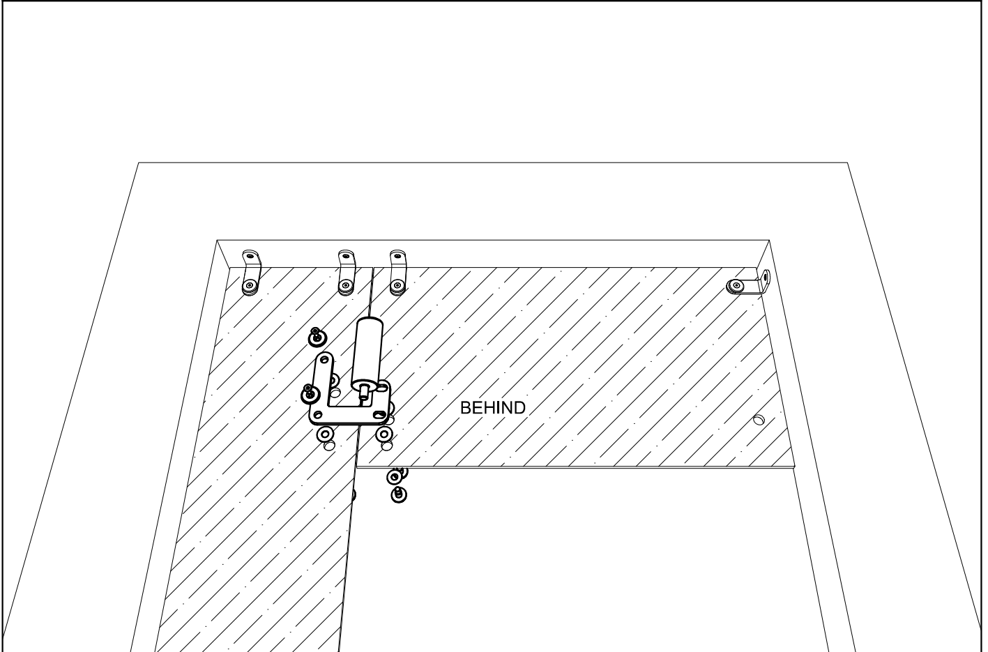
SC3-A.10 ZENITH SC3 - FIX THE INDICATED ACCESSORY
