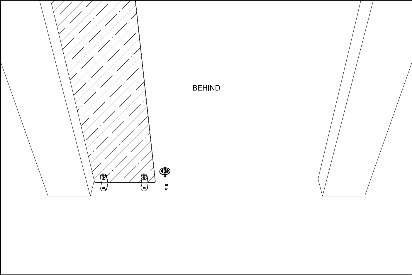
SC3-A.12 ZENITH SC3 -DRILL THE FLOOR AND ANCHOR THE BOTTOM ACCESSORY
