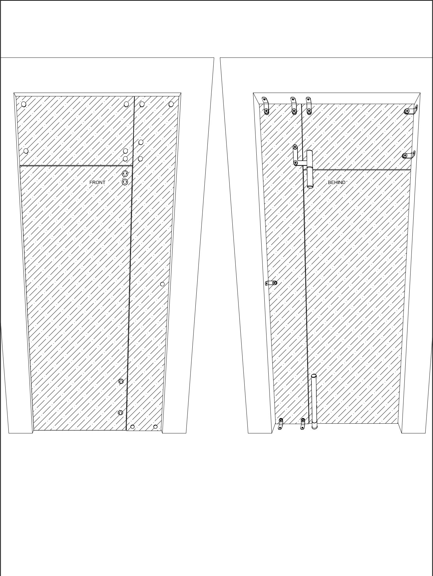
SC3-A.15 ZENITH SC3 - INSTALL THE REMAINING ACCESSORIES OF THE DOOR CLOSER AND THE WALL BRACKETS
